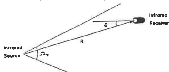
Figure 2 The Direct Path Optical Channel
