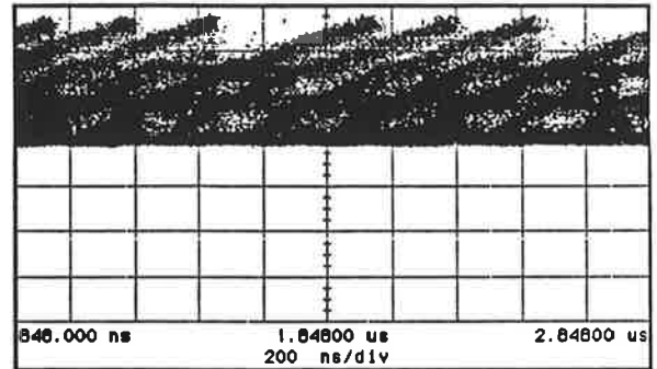
Figure 12 Detector Eye Pattern with Poor Carrier-to-noise Ratio (18.5 dB) Sufficient to Cause Loss of Clock.
