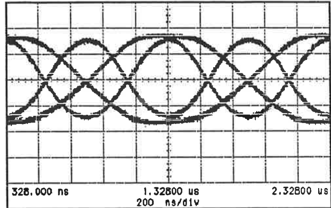
Figure 5 EYE Pattern of CSMK Baseband Signal
