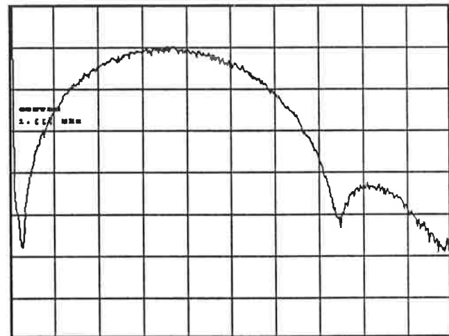
Figure 6 CSMK Baseband Spectrum at 1 Mb/s Data Rate. Display center = 1 MHz, X = 0.2 MHz/division, Y = 10 dB/division
