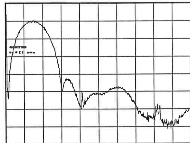
Figure 7 CSMK Baseband Spectrum with Display Sweeping Up To 5 MHz. X = 0.5 MHz/division
