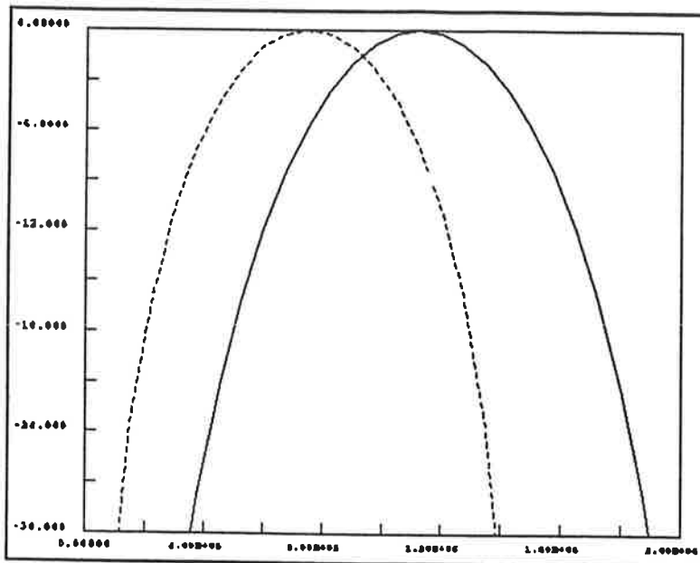
Figure 3 Power Density Spectrum for CMSK (solid line) and 3-level PR4 (dashed line)
