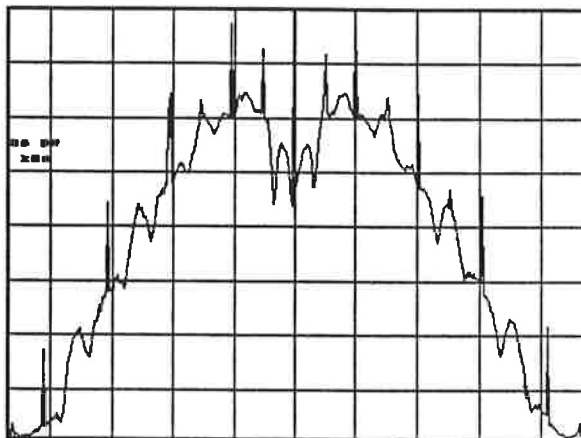
Figure 9 RF Spectrum at \pm 3 MHz Deviation.
