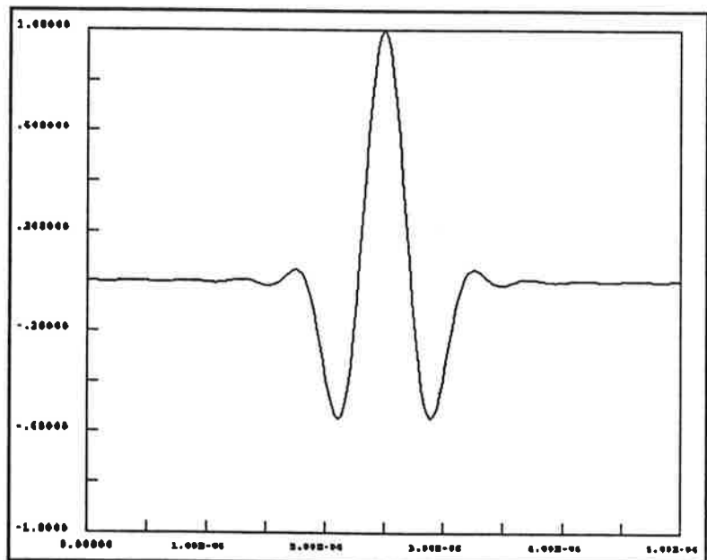
Figure 4 Generating Pulse Shape for CMSK
